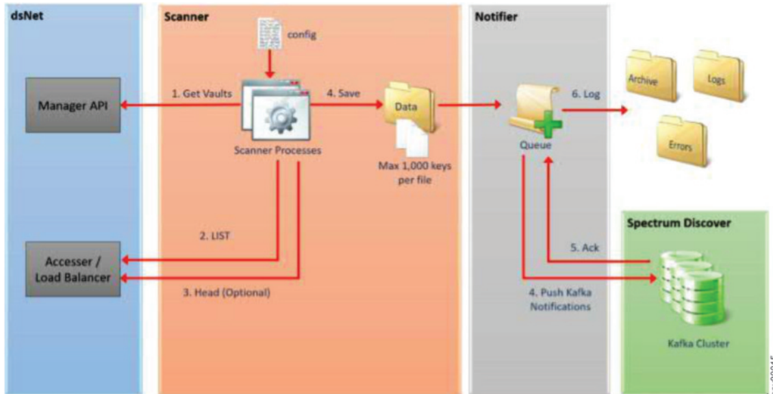
Figure 23. IBM Cloud Object Storage [Replay] architecture
