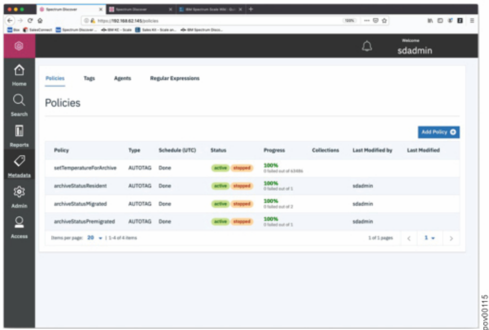
Figure 13. User-defined policies to assign values to Archive status tag
