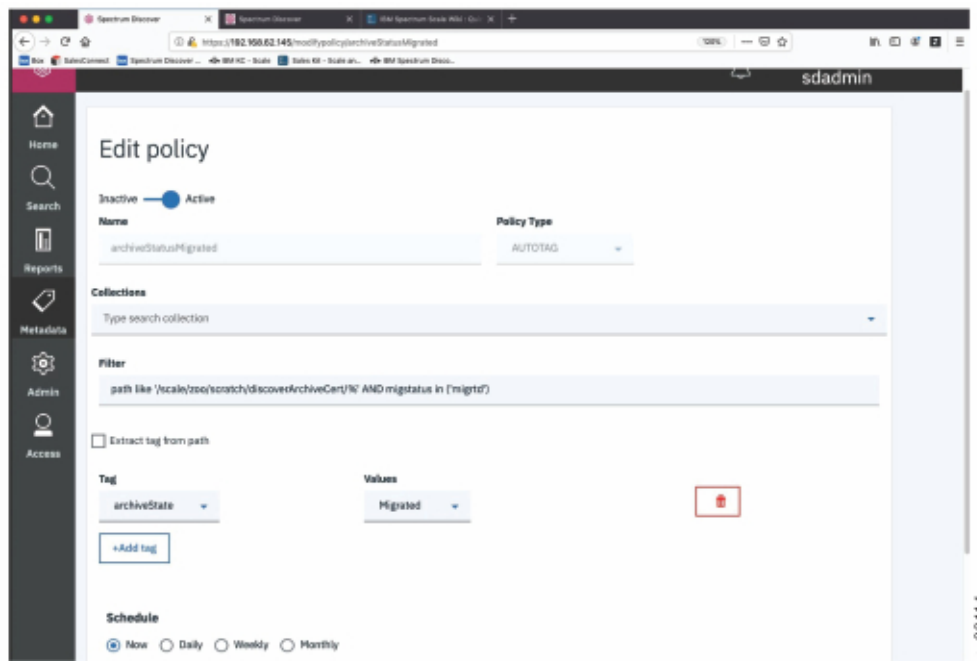
Figure 12. Policy defining archive tag value
