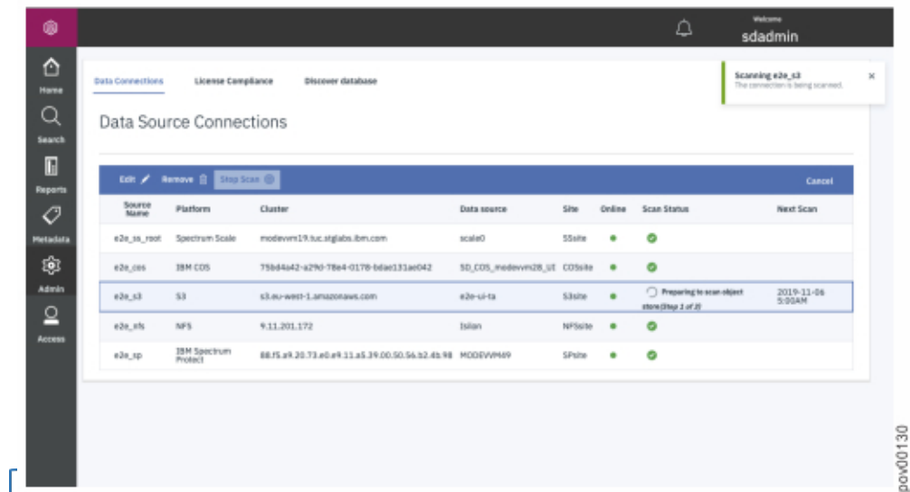
Figure 11. A scan in a state of Scanning
