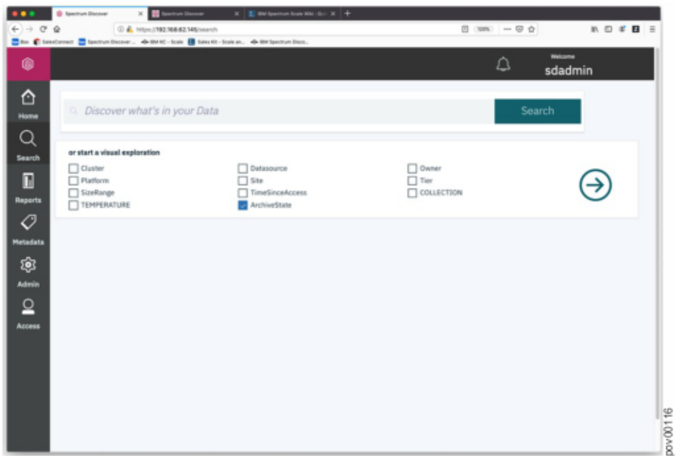
Figure 14. Visual exploration enabled for Archive state through the user-defined tag.
