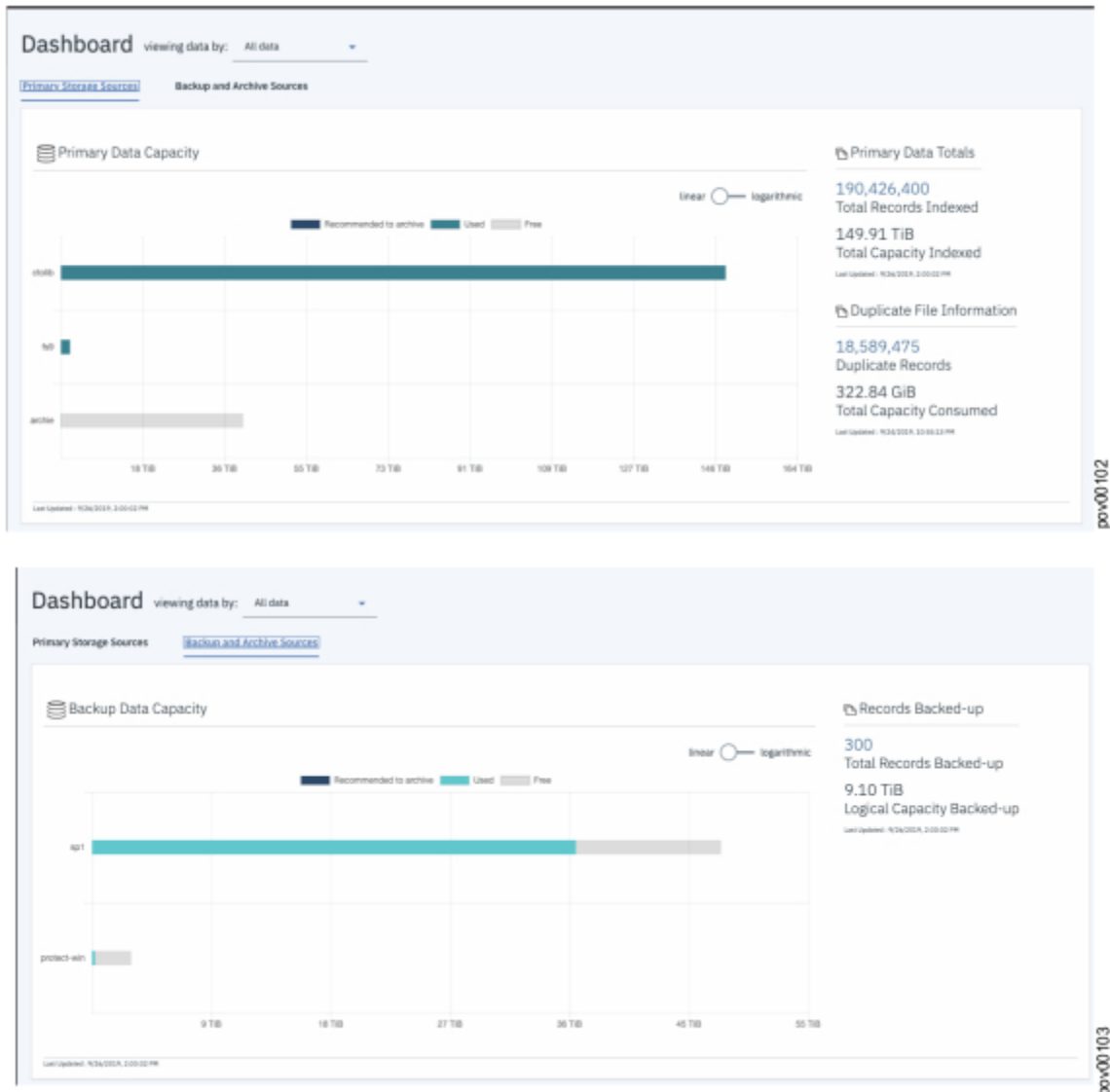
Figure 3. Example of the IBM Spectrum Discover dashboard
